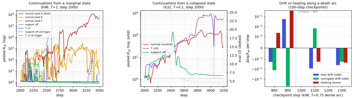
Figure 5: Left: continuations from a marginal k96/T1 state (step 2000); three normal seeds against support-off and T \times 3 , applied from the start (solid) or at a boundary-inflation trigger (dashed). Middle: continuations from a collapsed T=0.1 state; solid lines show scale, dotted lines evaluation CE. Right: the one-step decomposition along a dense death arc ( k96, T=0.75 , checkpoints every 100 steps; collapse at approximately step 960).
