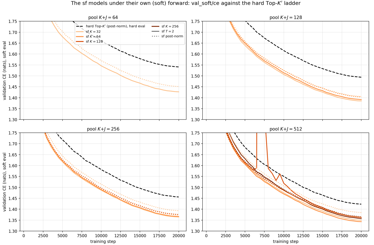
Figure 5: The soft family under its own forward ( val_soft/ce ), one panel per pool, against the pool-matched hard Top- K' baseline (dashed). Solid T = 2 , dotted post-norm. Every curve ends below the dashed reference; within a panel the curves cluster tightly across K .
