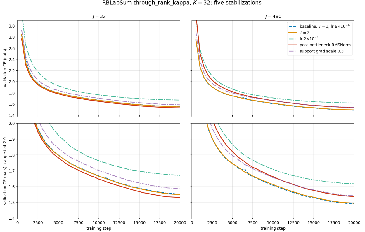
Figure 1: K = 32 : smaller candidate window on the left, larger on the right; the lower row repeats each panel with the vertical axis capped at 2.0 nats. Colour encodes the arm and line style its kind: the untouched baseline is dashed, the two arms that stabilize without an accuracy cost ( T = 2 and the output RMSNorm) are solid, and the two attenuating arms (reduced learning rate, support-gradient scale) are dash-dotted and slightly transparent. Every arm survives here, so this configuration measures cost rather than stabilization: the baseline and T = 2 curves are indistinguishable, the output RMSNorm wins at J = 32 but loses 0.047 nats at J = 480 , and the reduced learning rate is clearly behind throughout.
