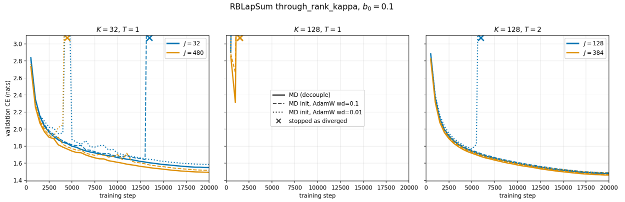
Figure 2: Validation CE for the RBLapSum through_rank_kappa family, panels as in the previous figure. In the middle panel every run of both (K, J) pairs diverges within the first \sim 2000 steps.
