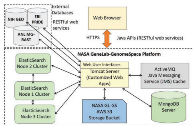
Fig. 4. GLDS system architectural components (customized GeneLab-GenomeSpace platform). Graphical representation of technical coordination between external databases and web browser to the GeneLab-GenomeSpace platform utilizing the MongoDB server and NASA AWS storage
