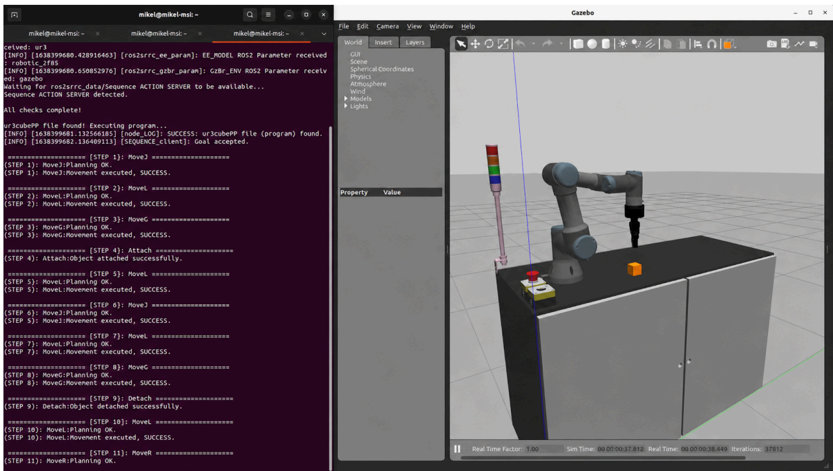
Figure 3.5: Universal Robots UR3 6-DOF collaborative manipulator with Robotiq 2F-85 gripper.
