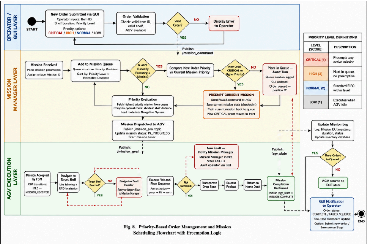
Figure 3.10: Priority-based order-management subsystem driving the PyQt5 industrial control centre.
