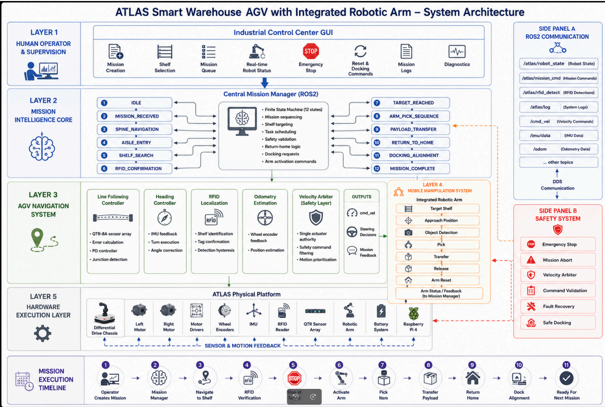
Figure 3.1: Overall system architecture of the ATLAS Smart Warehouse AGV with integrated UR3 arm.
