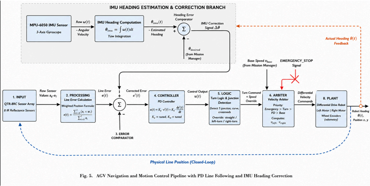
Figure 3.6: AGV motion-control pipeline using a Proportional-Derivative (PD) line-following controller.
