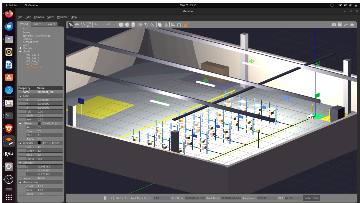
Figure 1.2: Conceptual warehouse layout showing aisles, shelves and the spine path used by the AGV.
