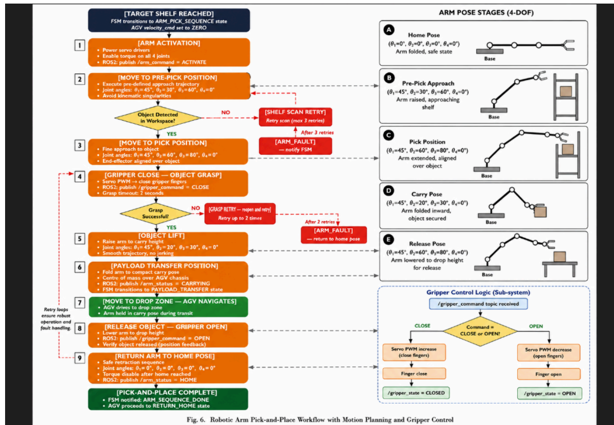
Fig. 6. Robotic Arm Pick-and-Place Workflow with Motion Planning and Gripper Control
