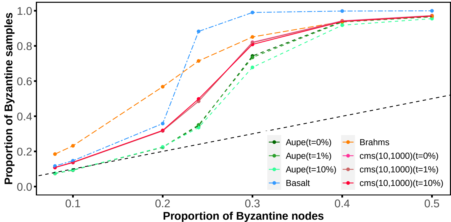
Resilience of strategies depending on f N=10000 v=160 F=10 sm=100 m=10
