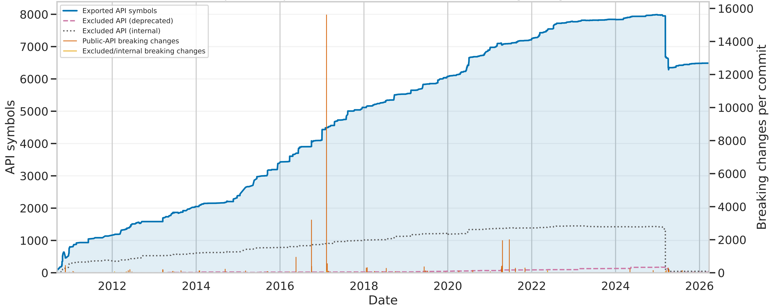
assertj-core: exported API, excluded API, and breaking changes
