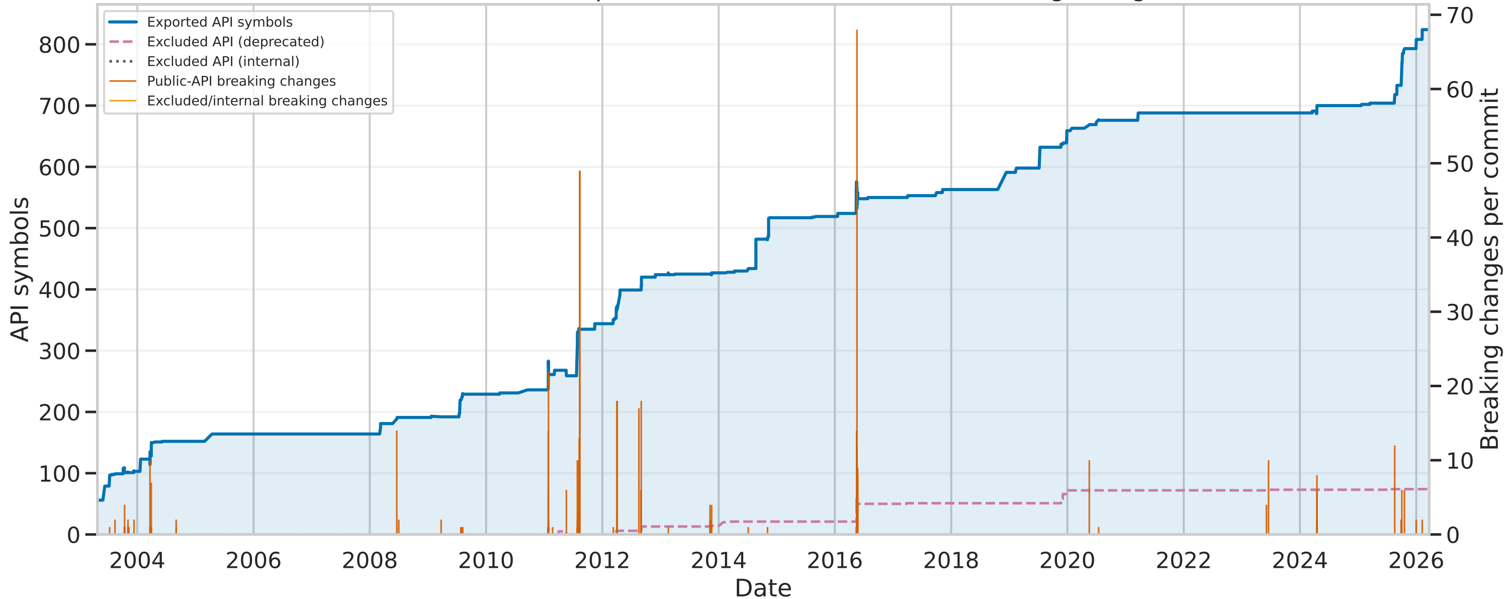
commons-codec: exported API, excluded API, and breaking changes
