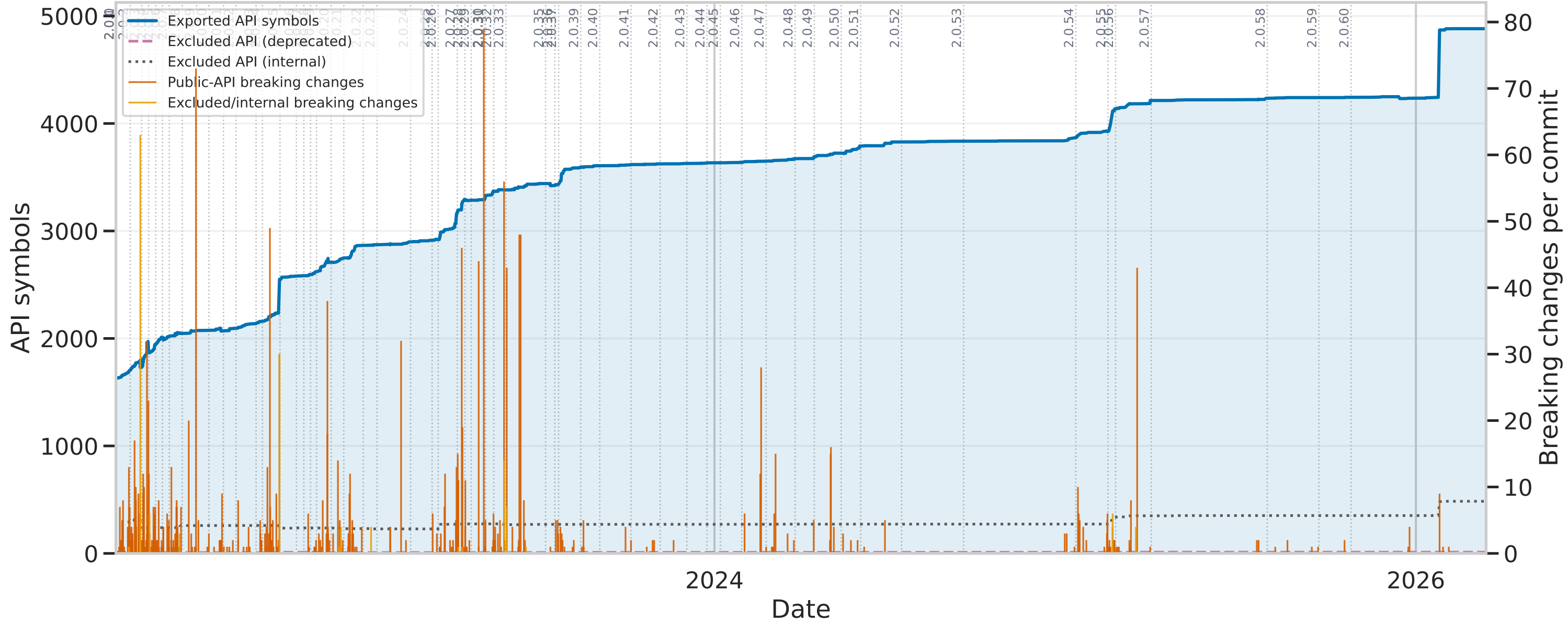
fastjson: exported API, excluded API, and breaking changes
