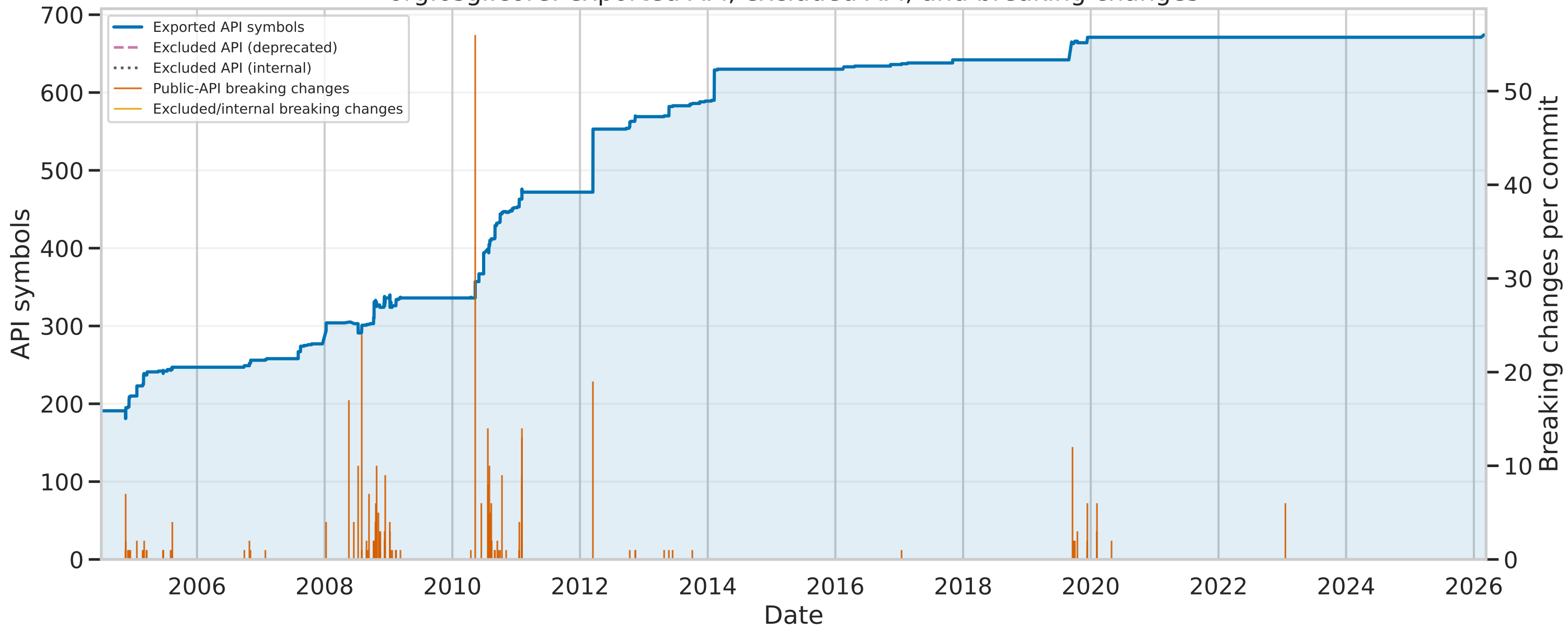
org.osgi.core: exported API, excluded API, and breaking changes
