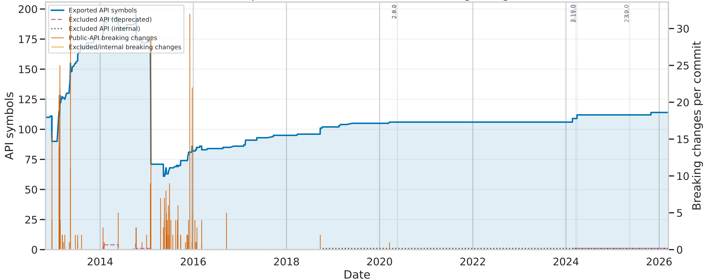
retrofit: exported API, excluded API, and breaking changes
