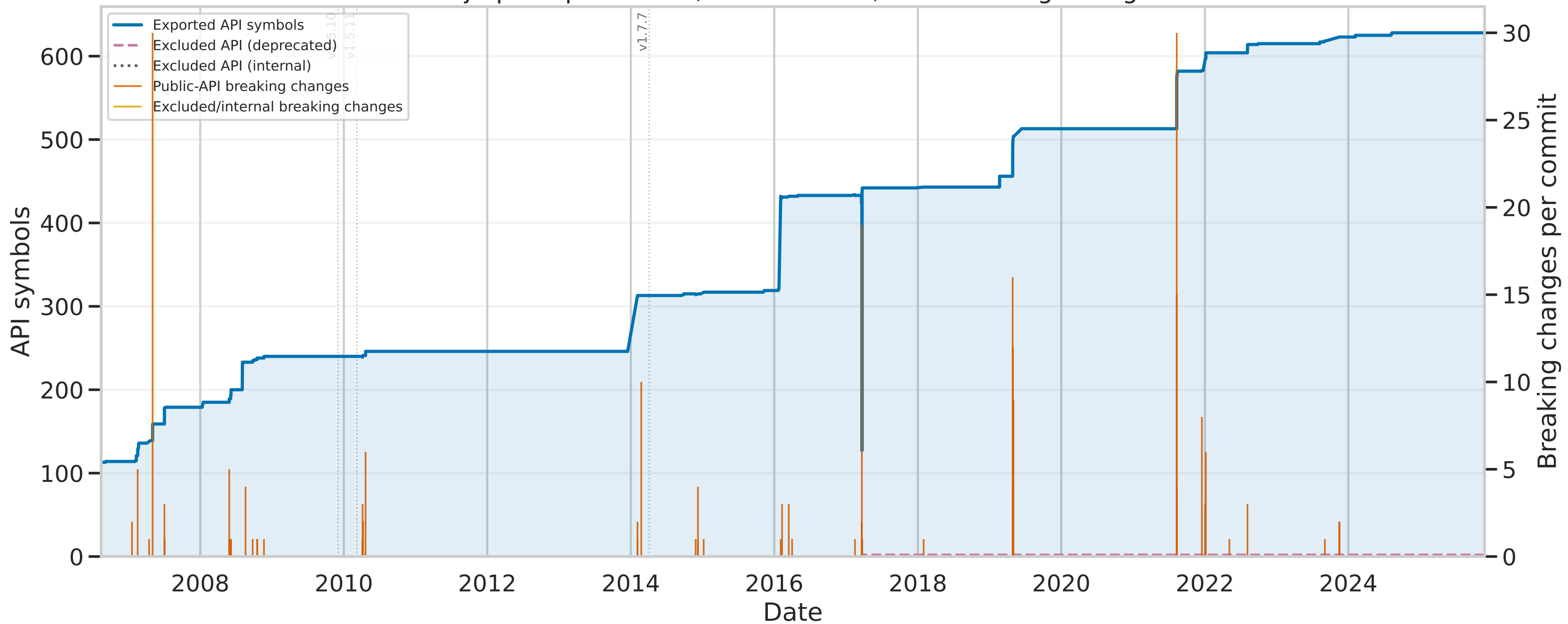
slf4j-api: exported API, excluded API, and breaking changes
