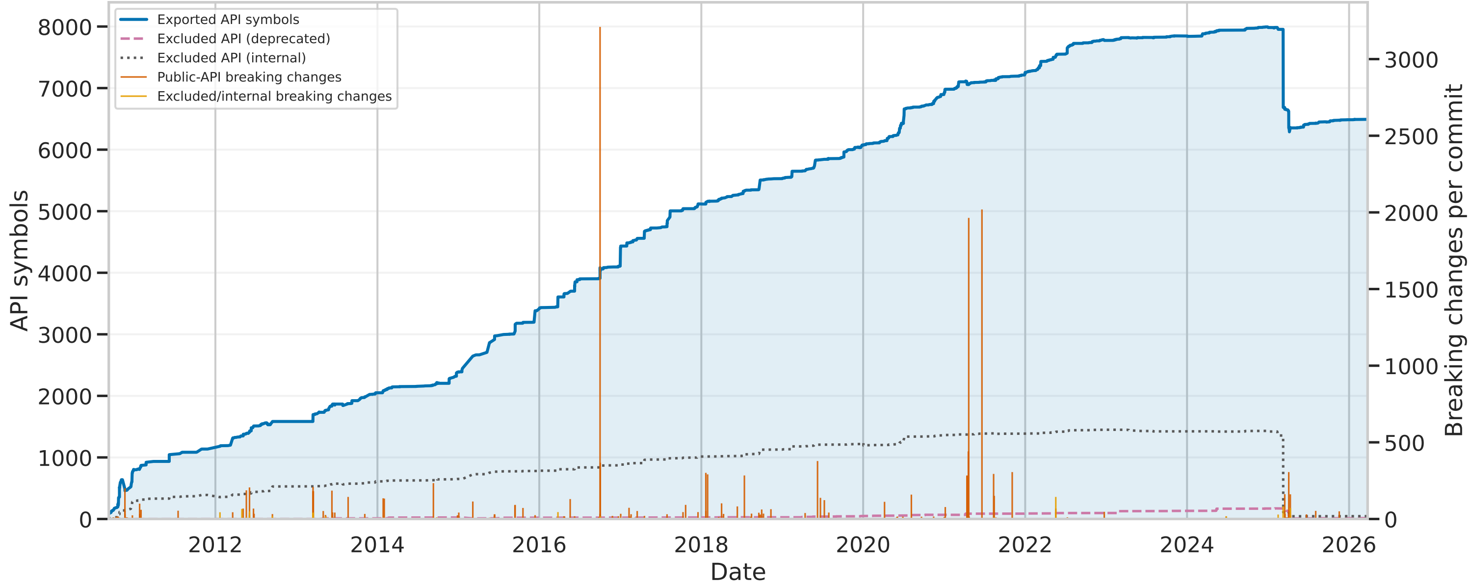
assertj-core: exported API, excluded API, and breaking changes
