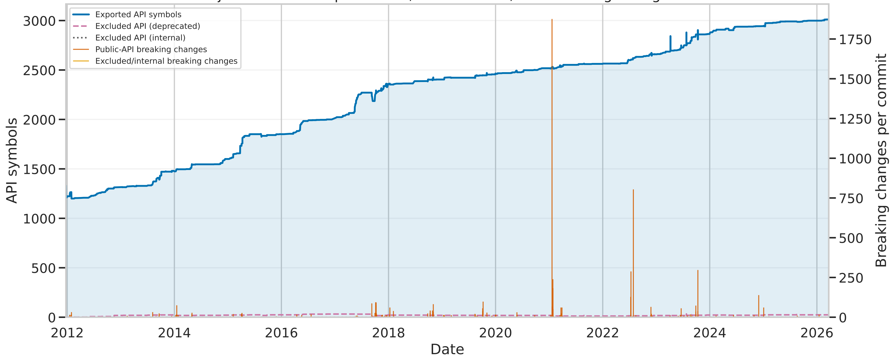
jackson-core: exported API, excluded API, and breaking changes
