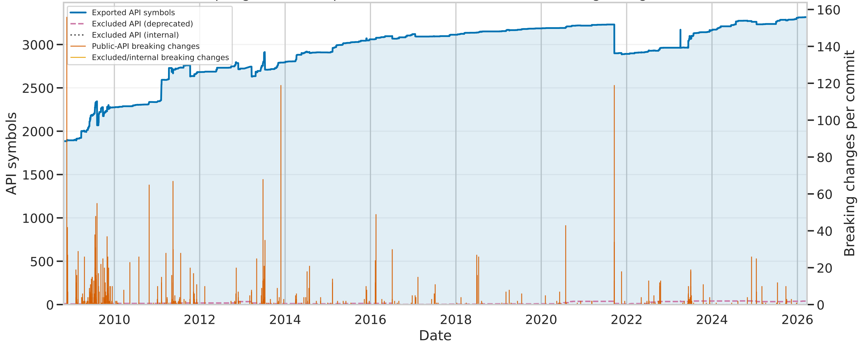
spring-context: exported API, excluded API, and breaking changes
