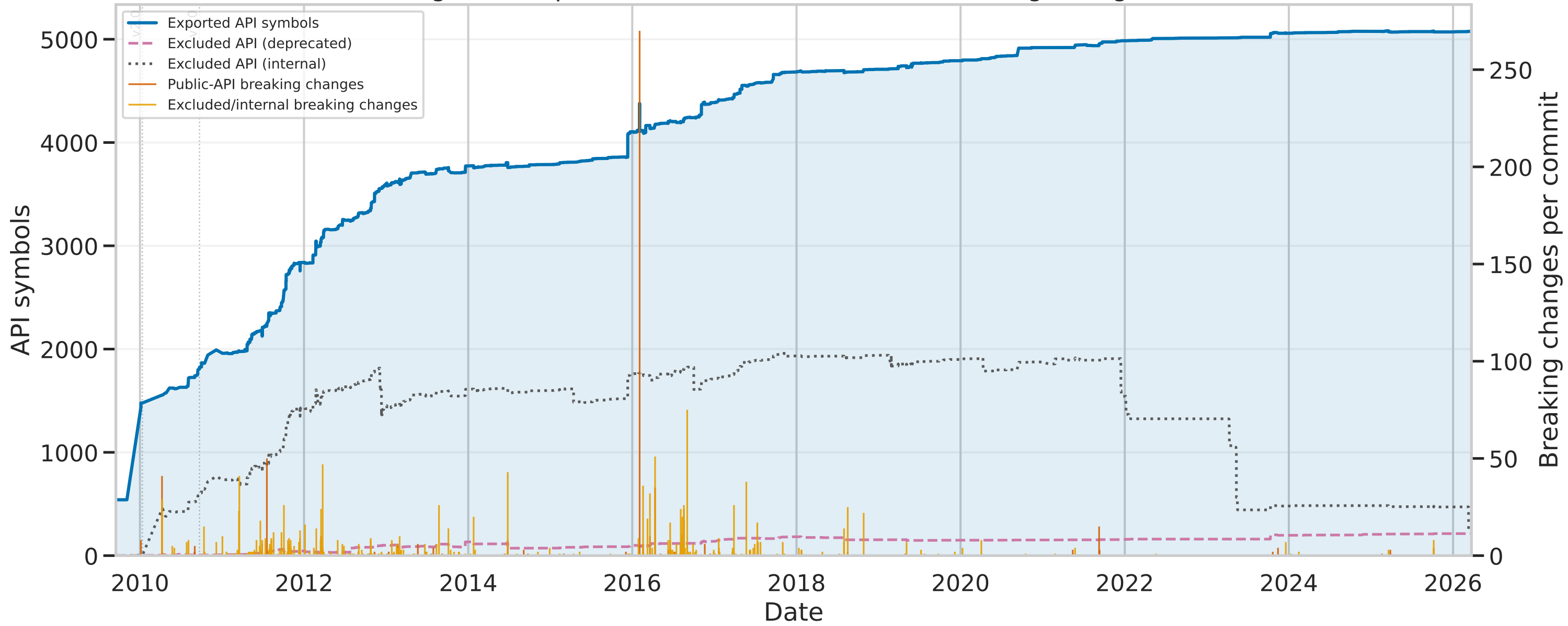
guava: exported API, excluded API, and breaking changes
