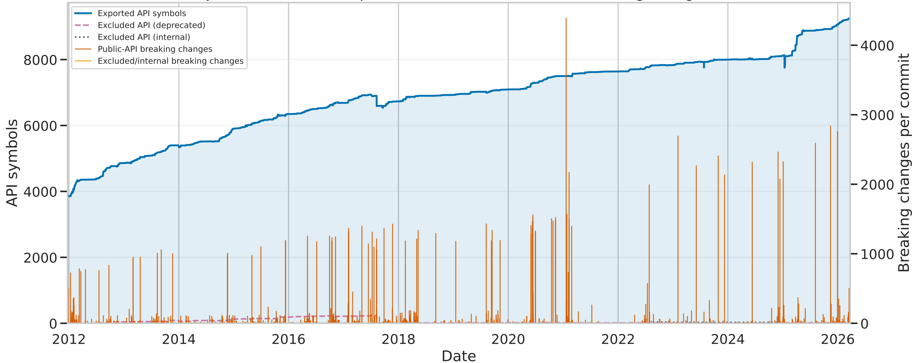
jackson-databind: exported API, excluded API, and breaking changes
