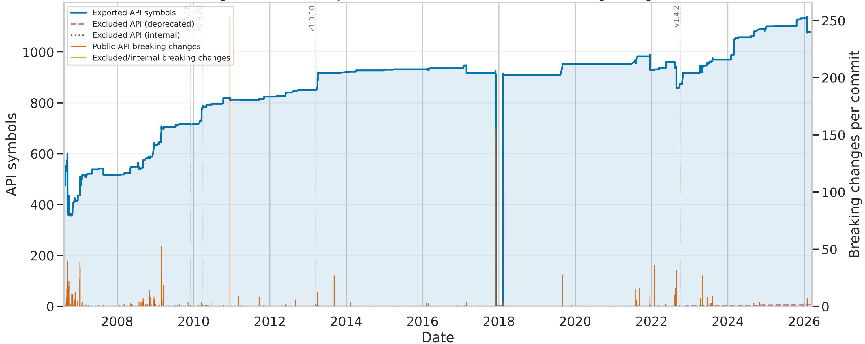
logback-classic: exported API, excluded API, and breaking changes
