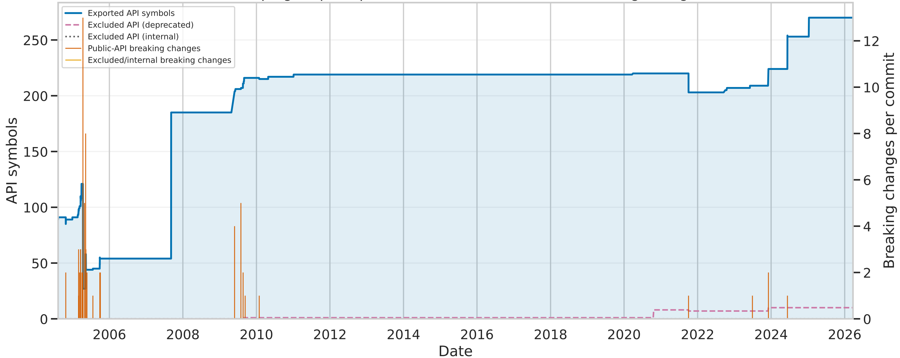
maven-plugin-api: exported API, excluded API, and breaking changes
