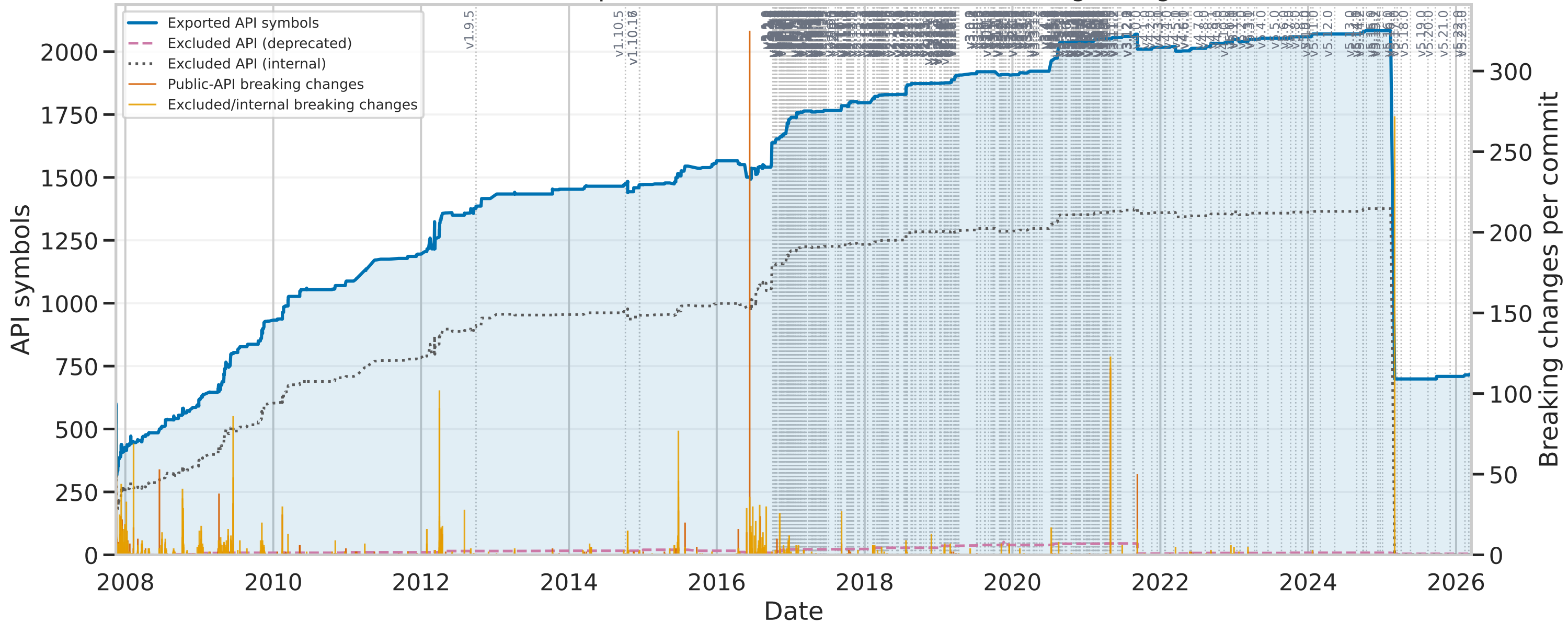
mockito-core: exported API, excluded API, and breaking changes
