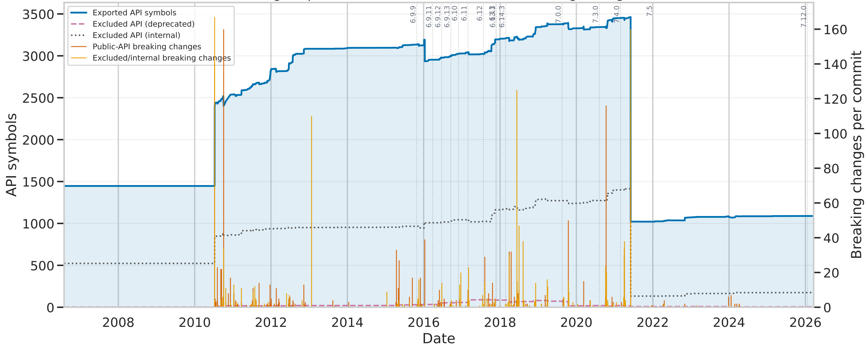
testng: exported API, excluded API, and breaking changes
