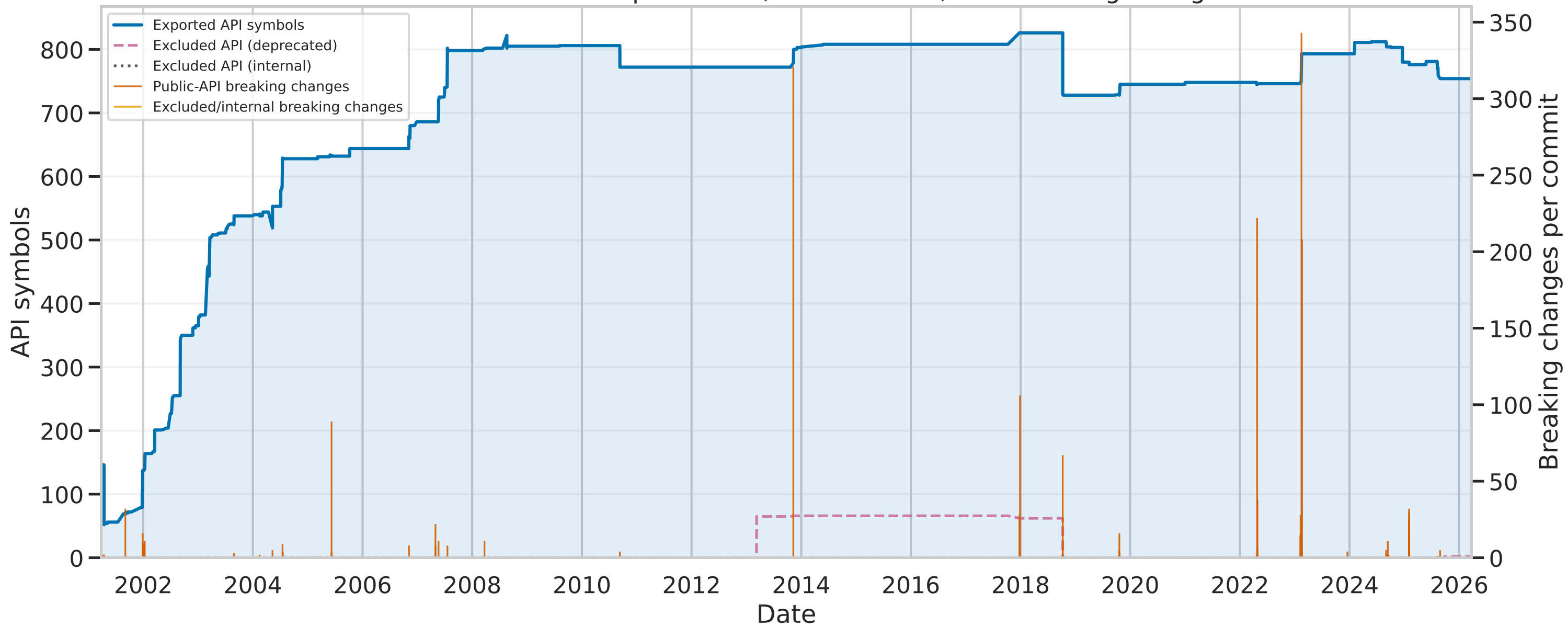
commons-beanutils: exported API, excluded API, and breaking changes
