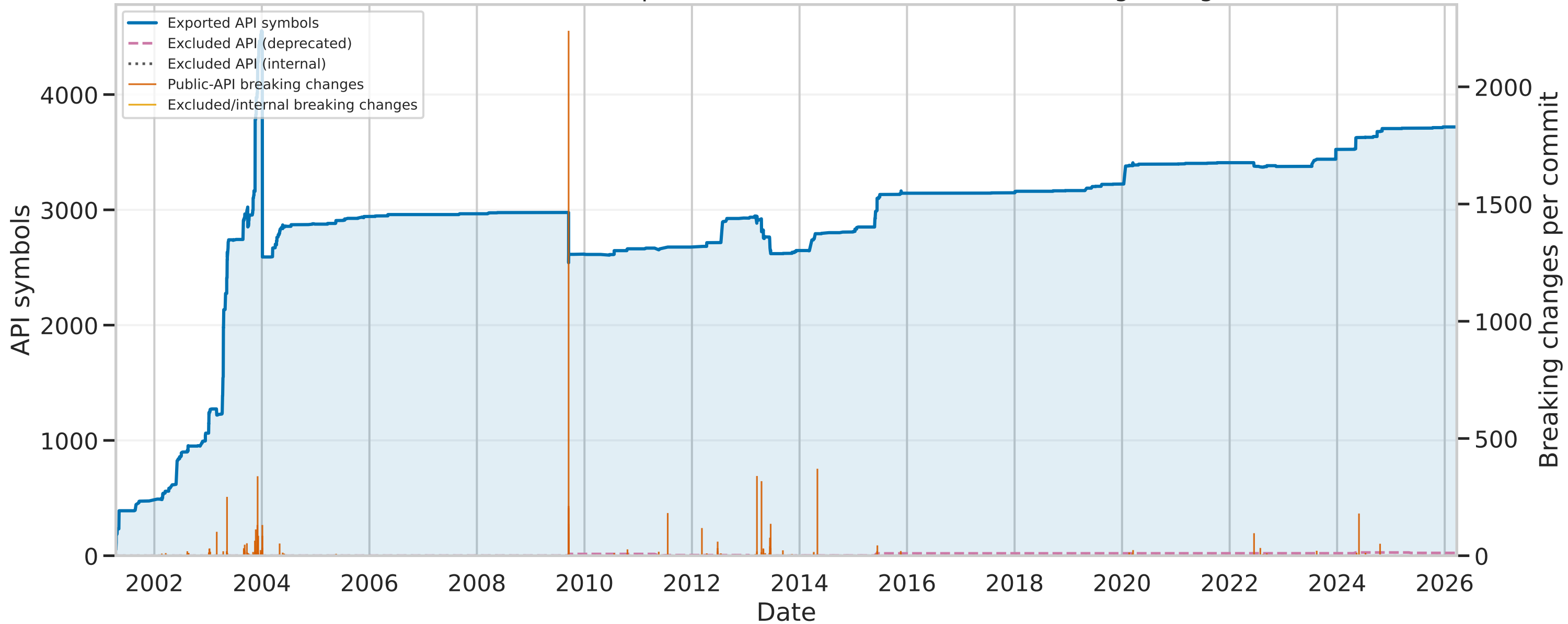
commons-collections: exported API, excluded API, and breaking changes
