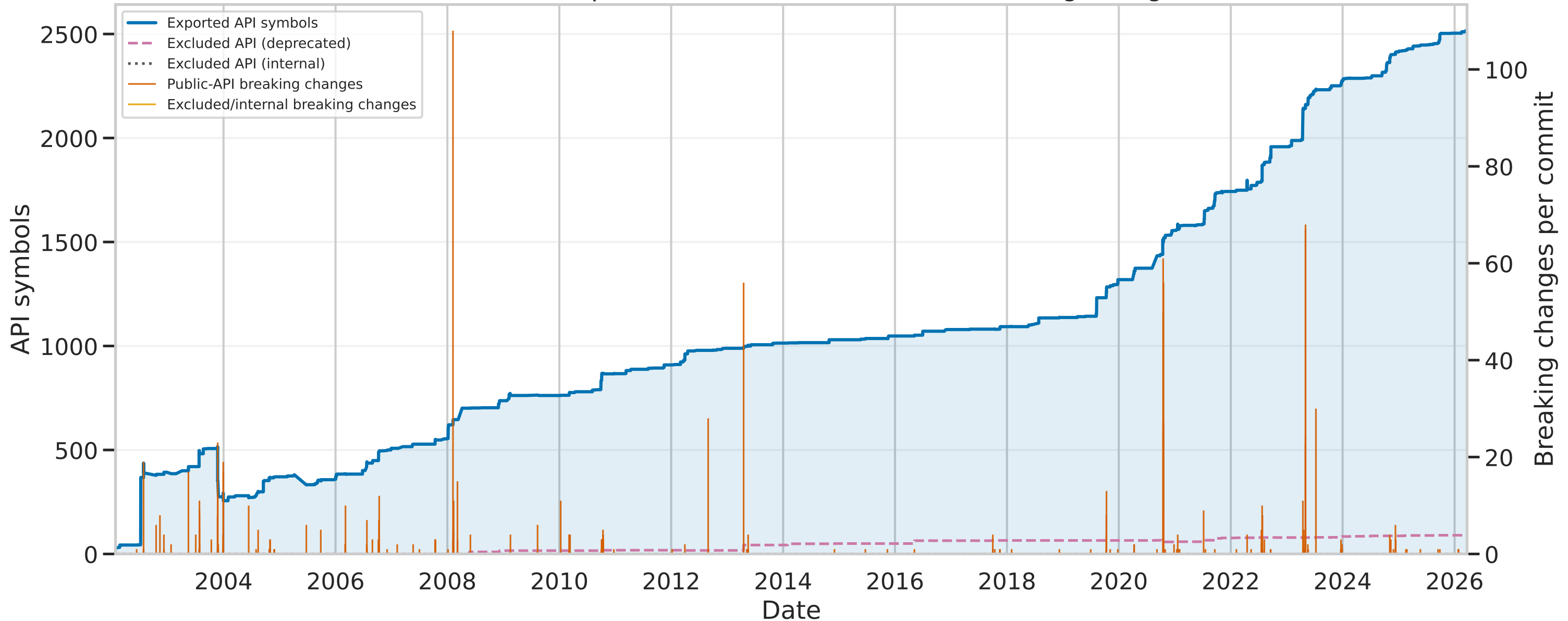
commons-io: exported API, excluded API, and breaking changes
