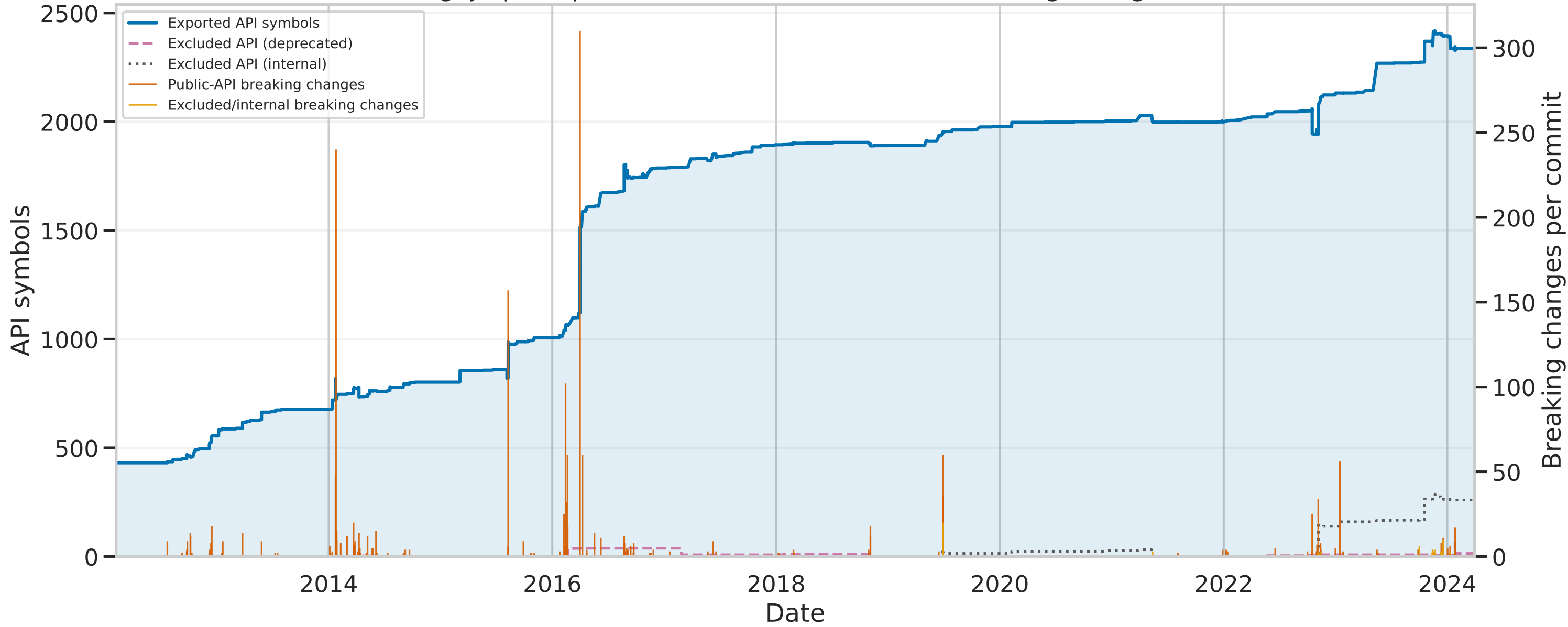
log4j-api: exported API, excluded API, and breaking changes
