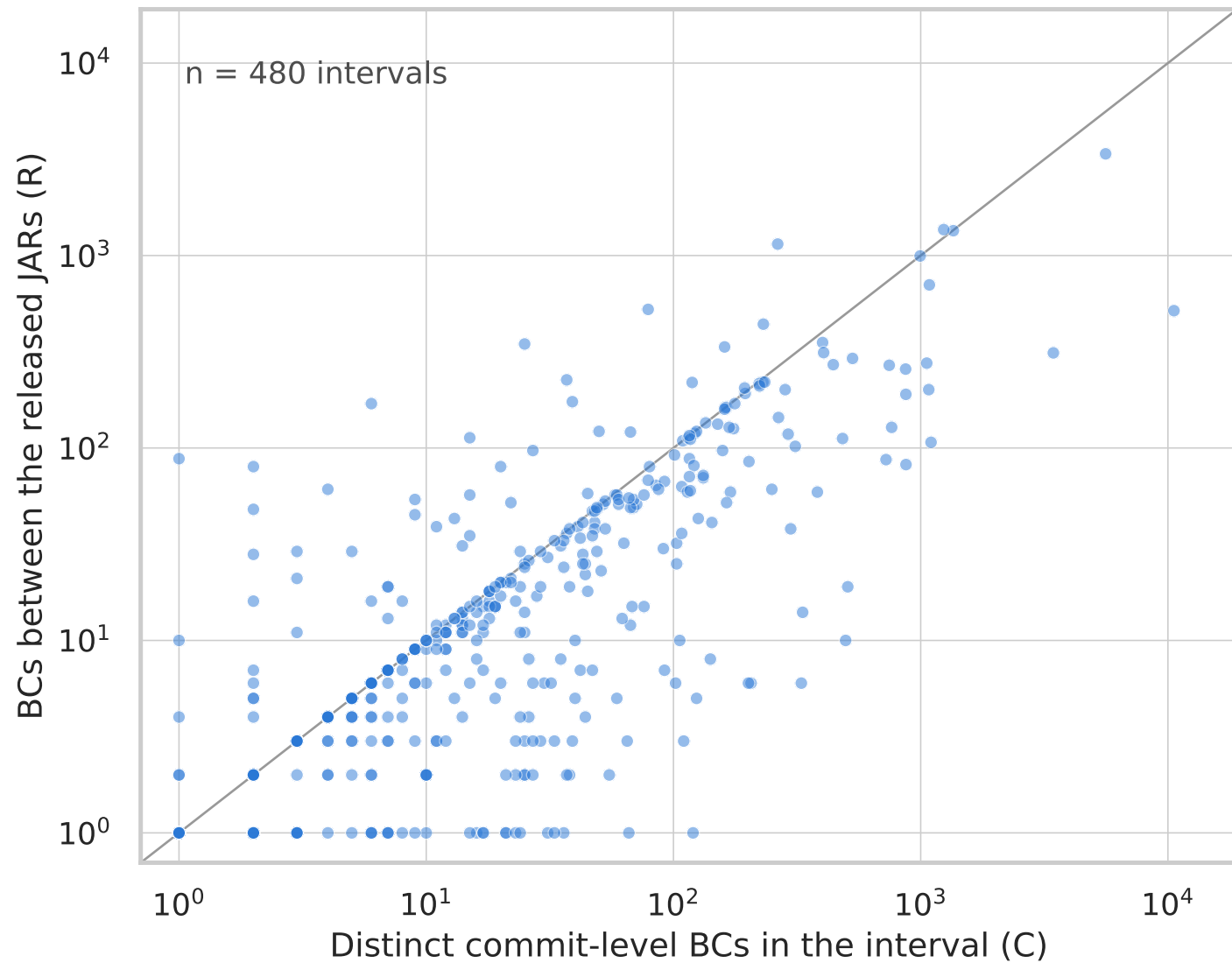
Commit level vs. release
