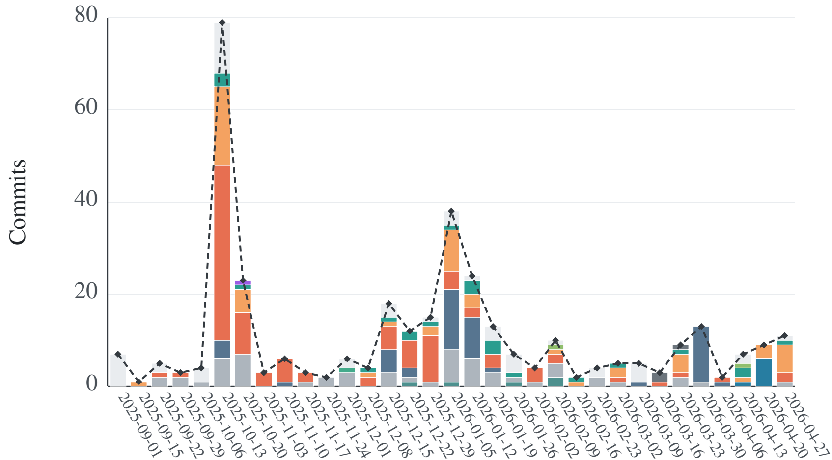
Commit Types Over Time — agent:amp
