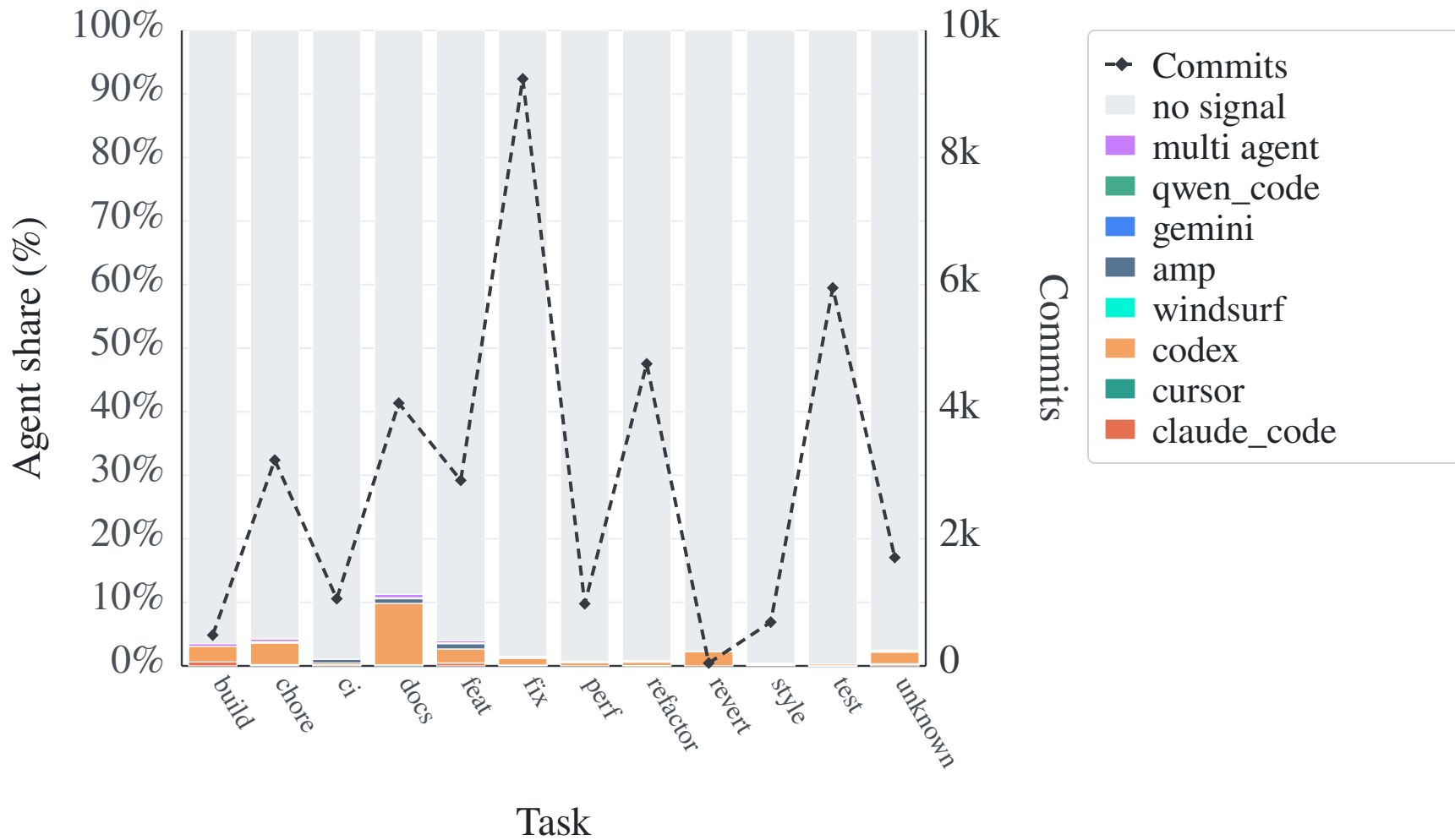
Agent Distribution by Task — steipete
