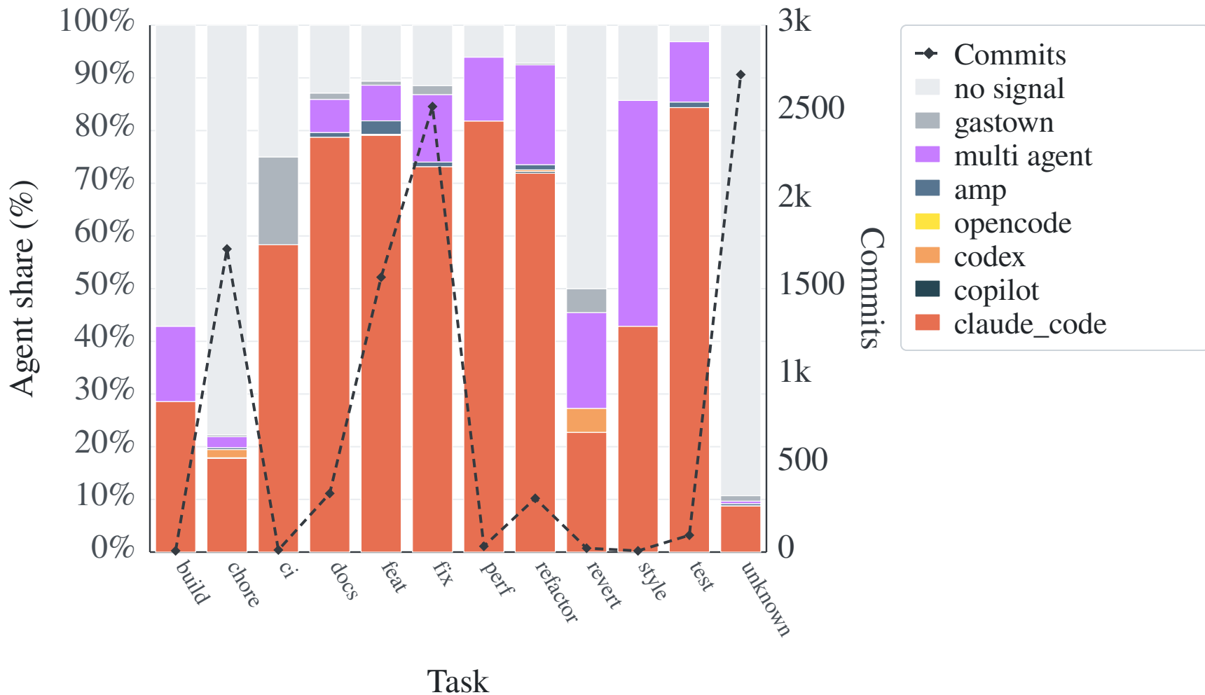
Agent Distribution by Task — steveyegge
