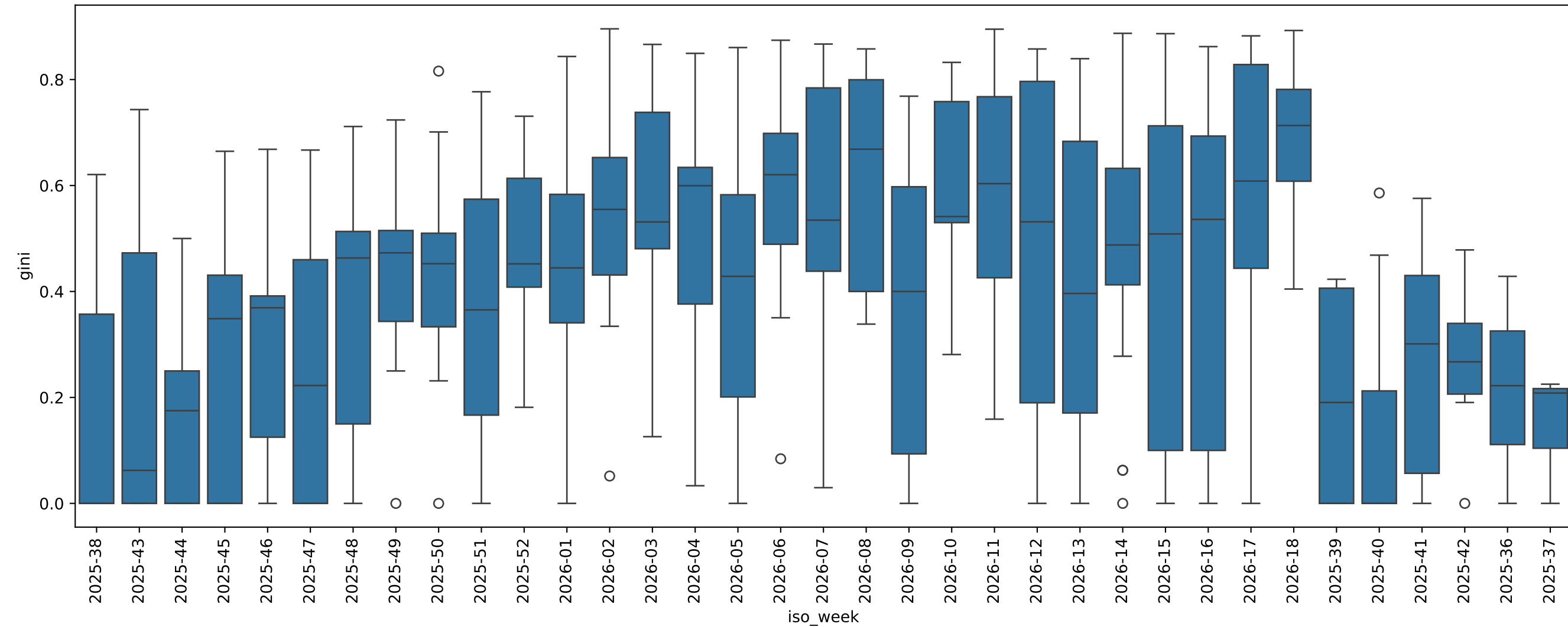
Repository concentration (Gini) per week (distribution across developers)
