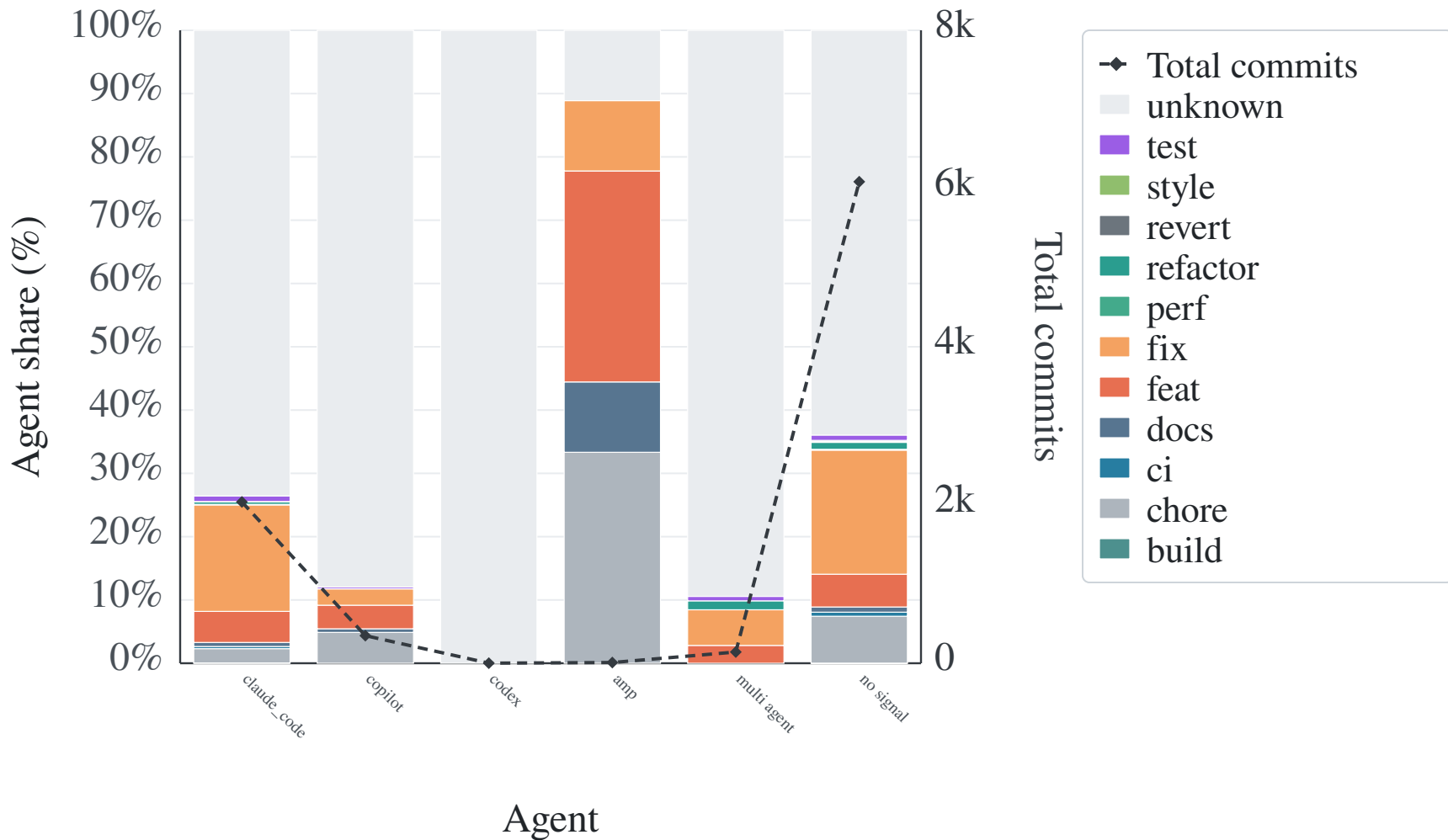
Commit Type Distribution by Agent — clubanderson
