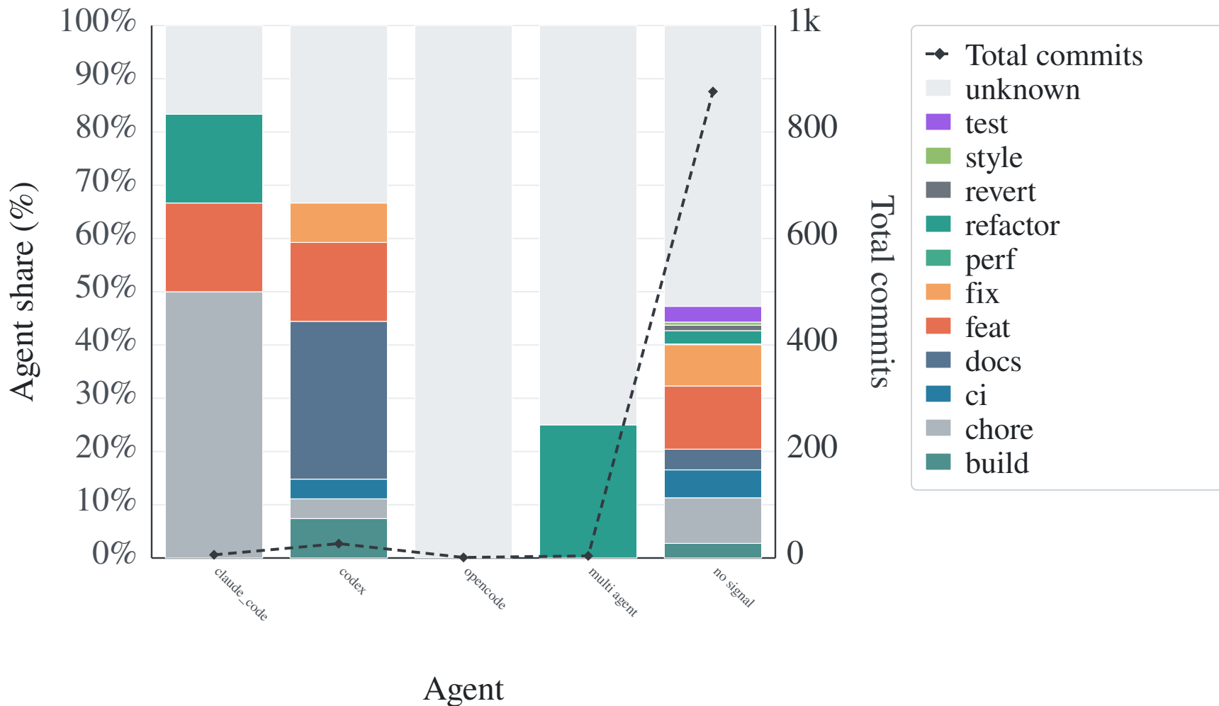
Commit Type Distribution by Agent — philipp-spiess
