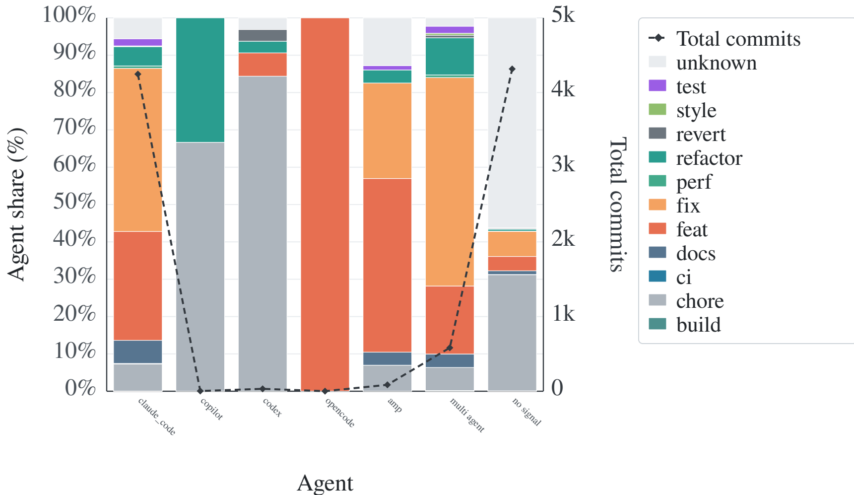
Commit Type Distribution by Agent — steveyegge
