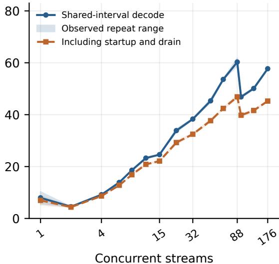
Aggregate tokens/s
