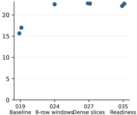
Whole-phase tokens/s
