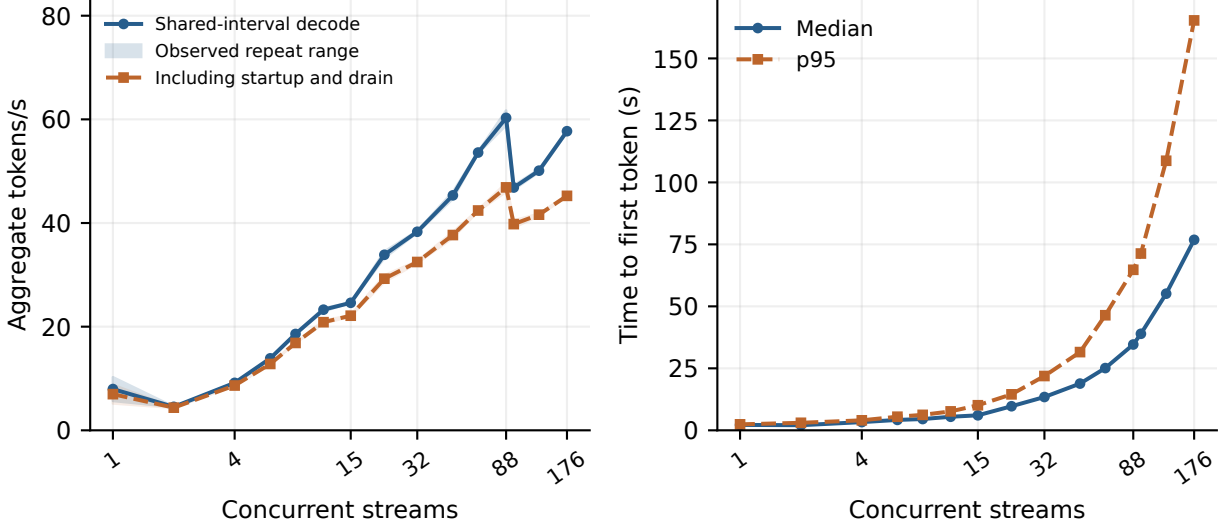
Figure 4: Paired measurements across fifteen concurrency levels. Left: common-interval decode throughput and whole-phase throughput, with shading showing the two observed phase rates. Right: pooled request TTFT median and 95th percentile. The 88-stream point is the highest paired mean on the measured grid.
