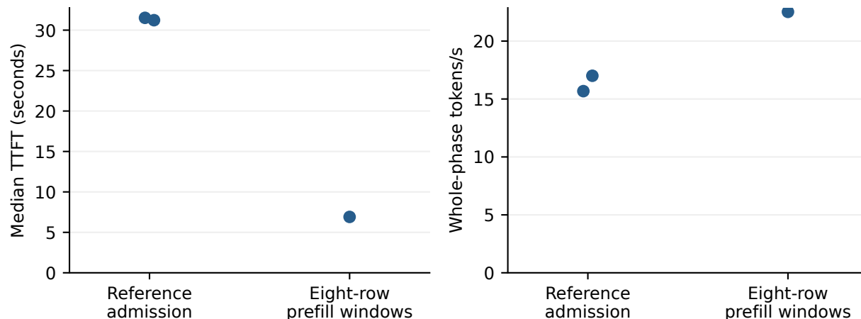
Figure 5: Fifteen-request bursts with an output cap of 128: reference admission and eight-row prefill windows. Each point is a retained phase. The comparison reports observed configurations with different prompt tags.
