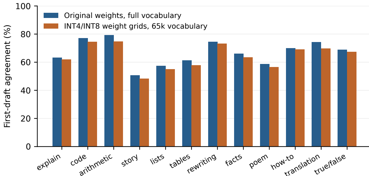
Figure 6: First-draft agreement by task family on captured fleet states. Each family contains three sequences. The two calculations share the same prediction targets and differ in draft weights and vocabulary.
