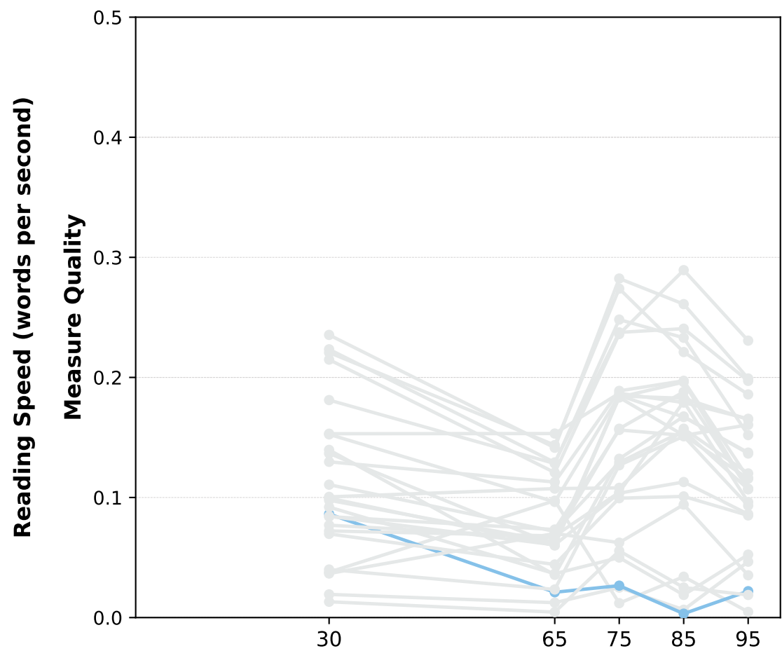
Sentences
