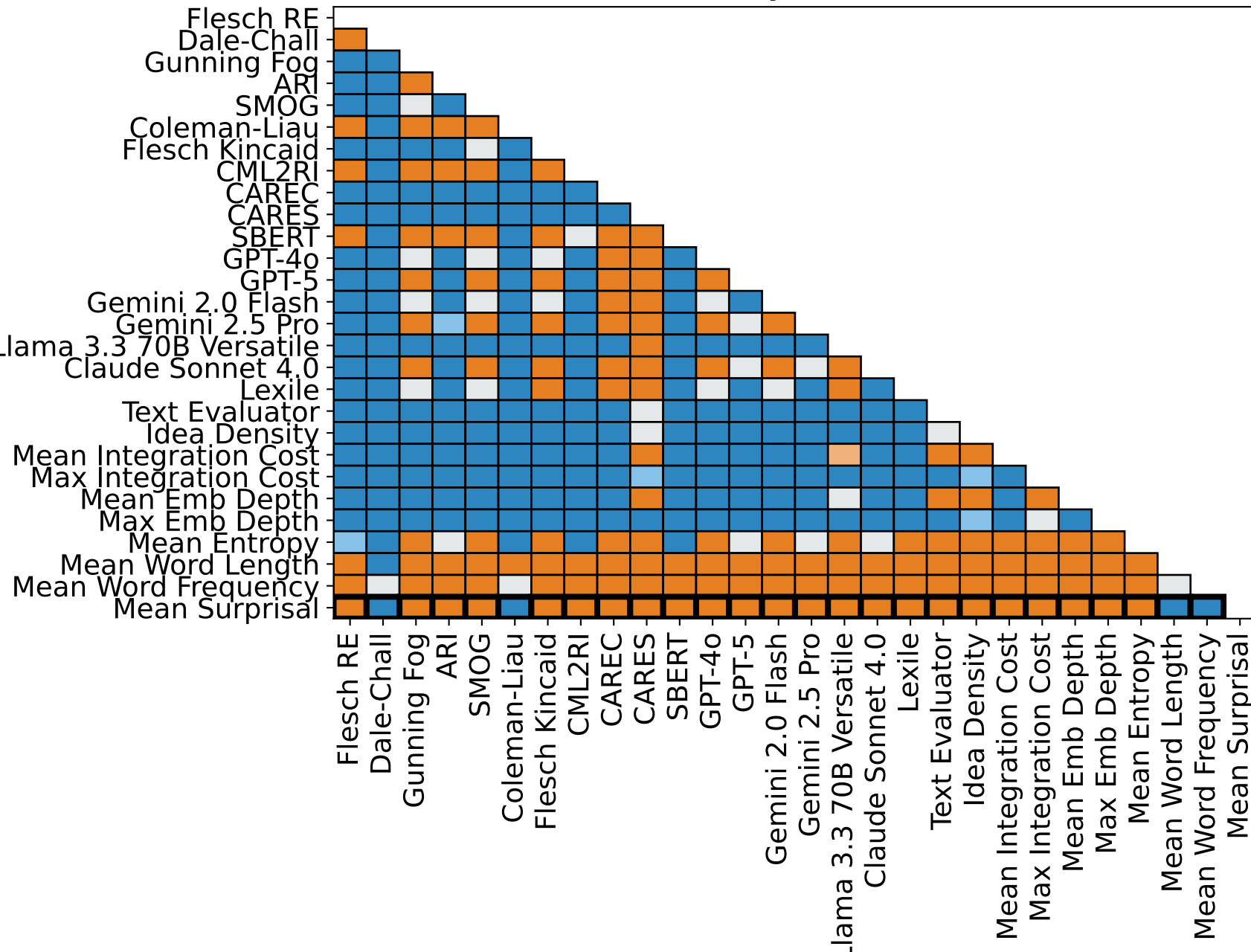
Regression Rate
