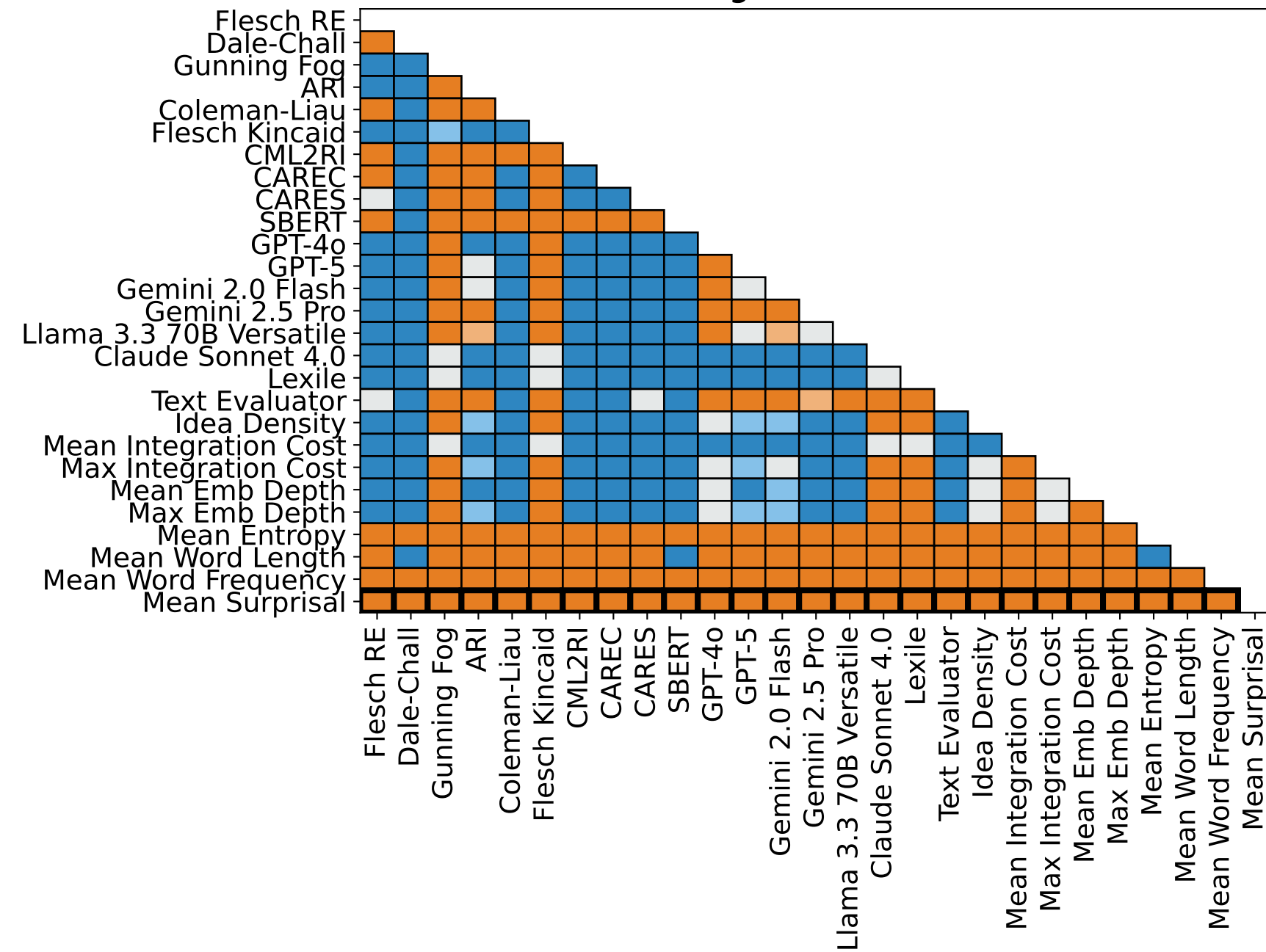
Regression Rate
