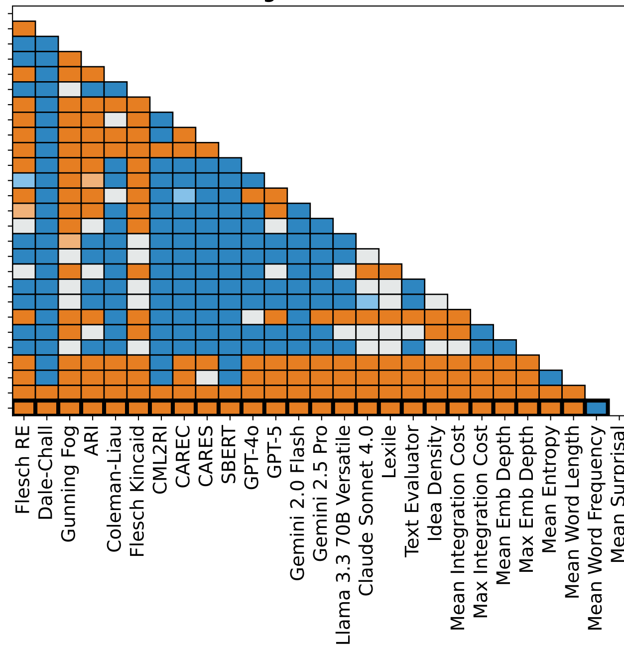
Regression Rate
