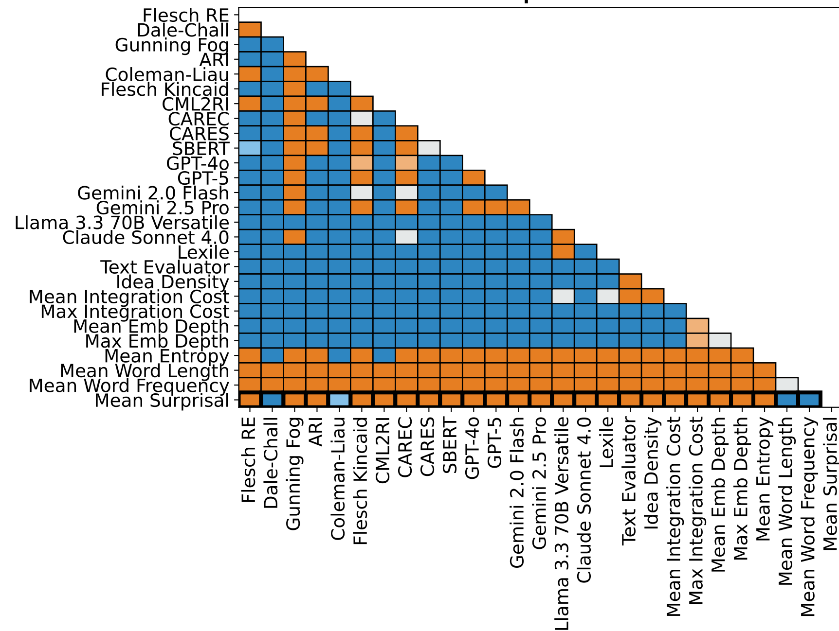
Regression Rate
