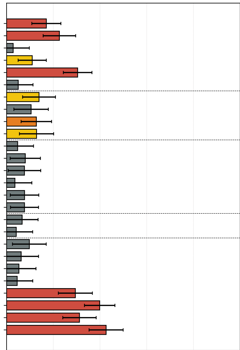
Skip Rate
