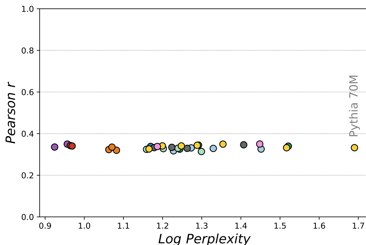
Regression Rate
