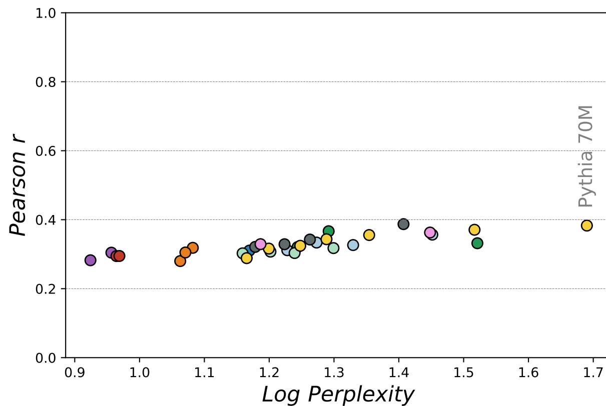
Sentences
