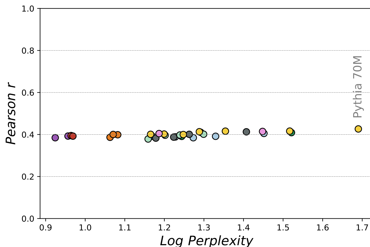
Skip Rate
