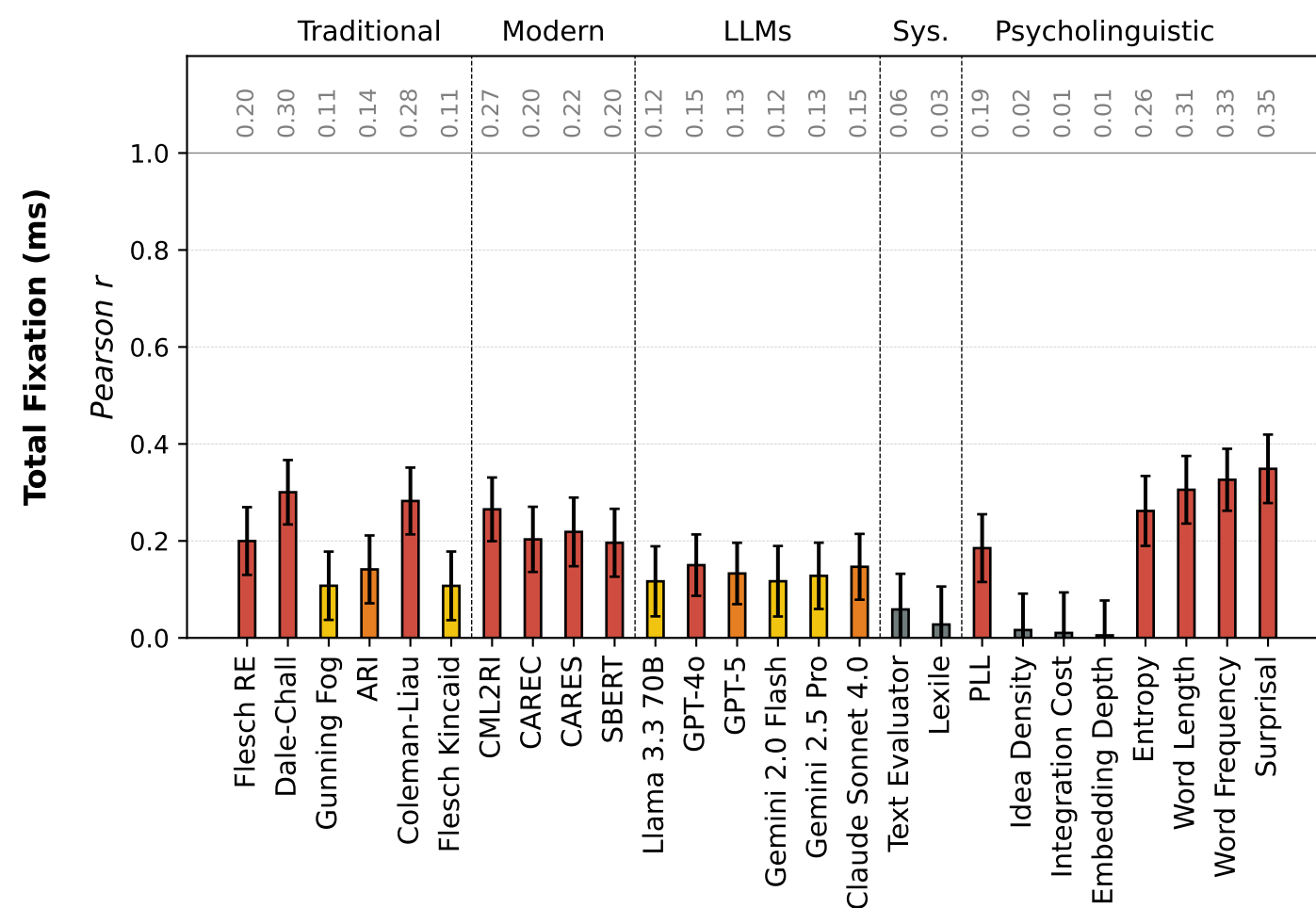
Sentences
