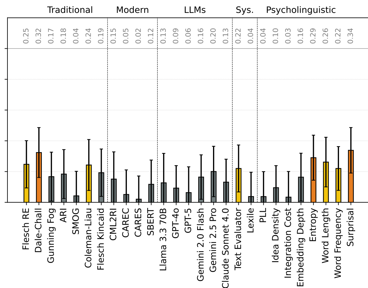
Paragraphs
