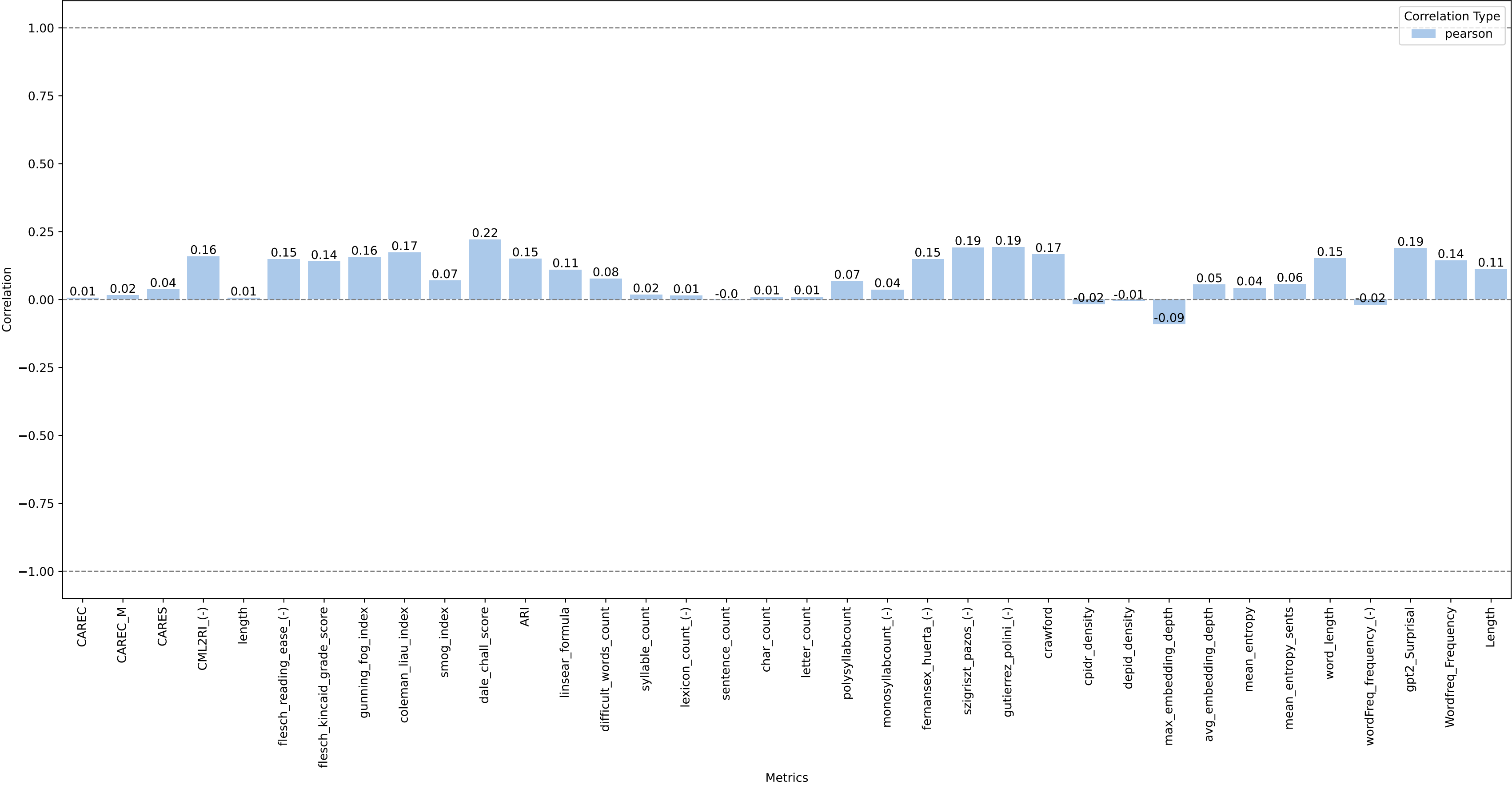
Correlation between Metric Differences and TF Differences | Alignment Resolution: paragraph remove outliers: False
