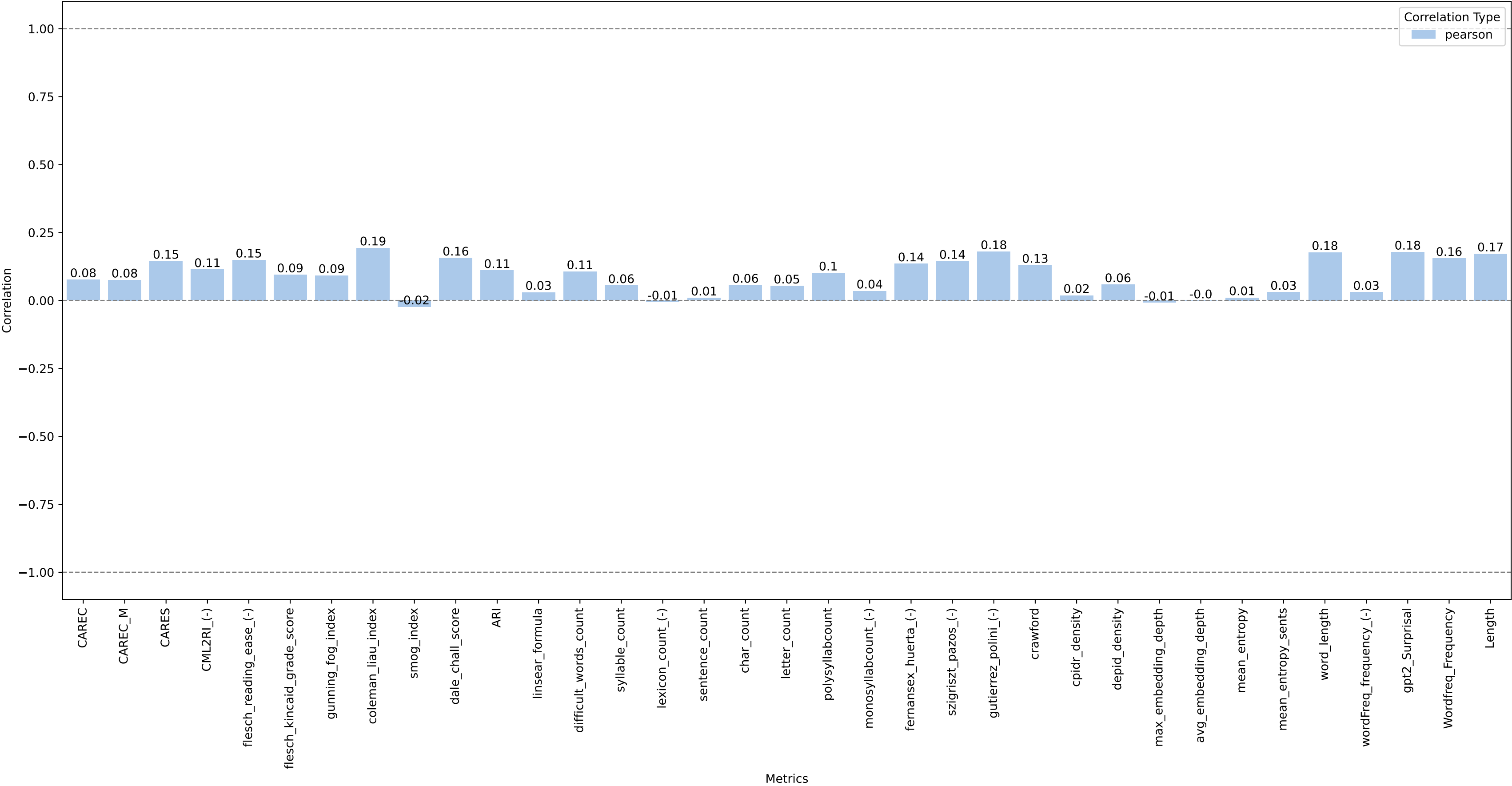
Correlation between Metric Differences and TF Differences | Alignment Resolution: sentence
