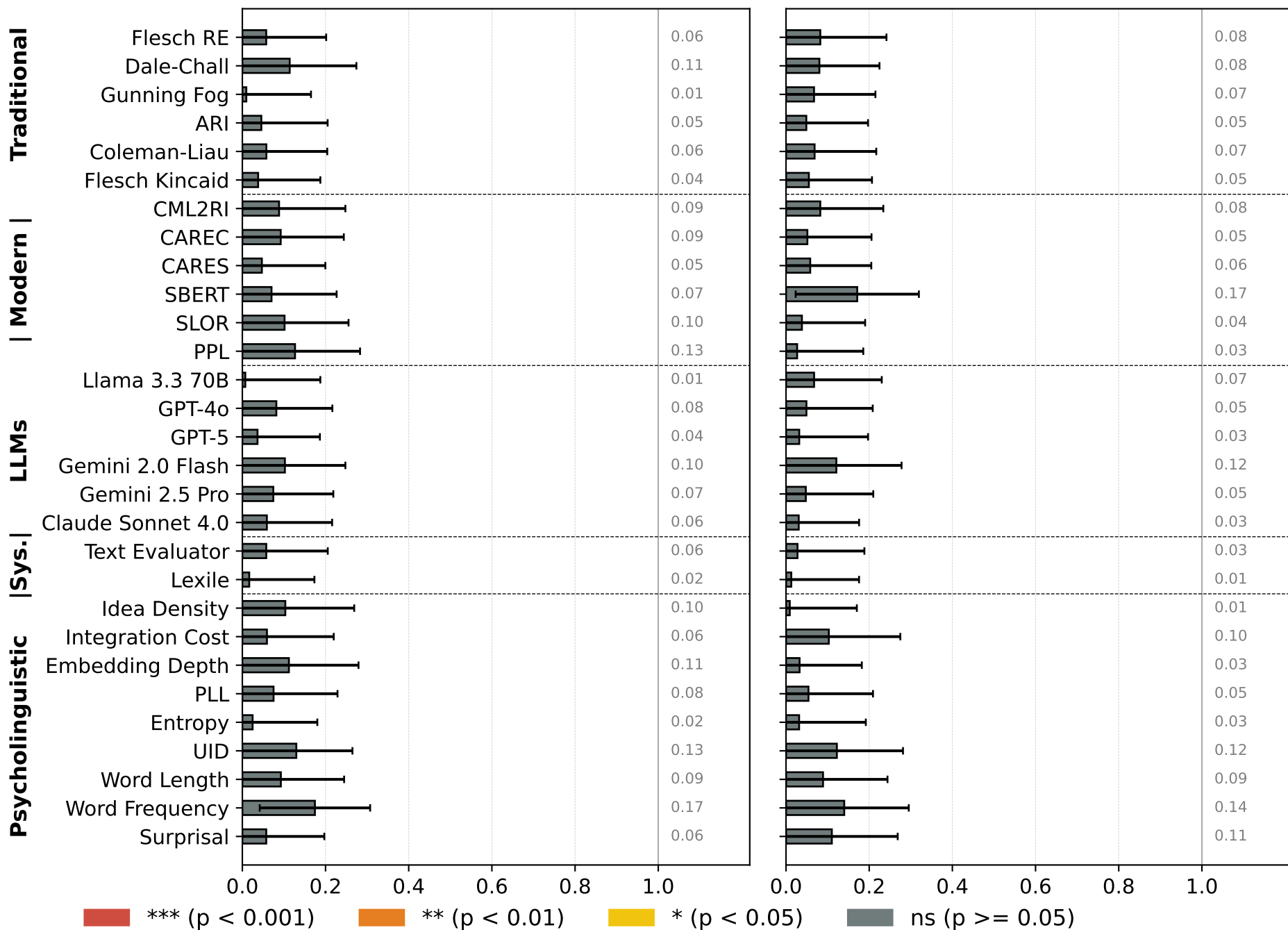
Comprehension Accuracy
