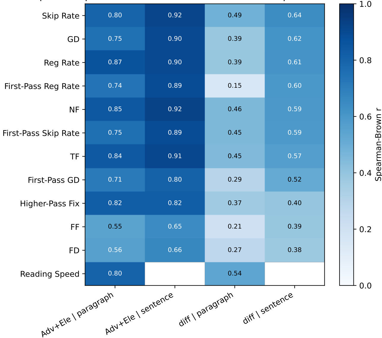
Split-half Spearman-Brown r — main+sm metrics — pearson — N=1000
