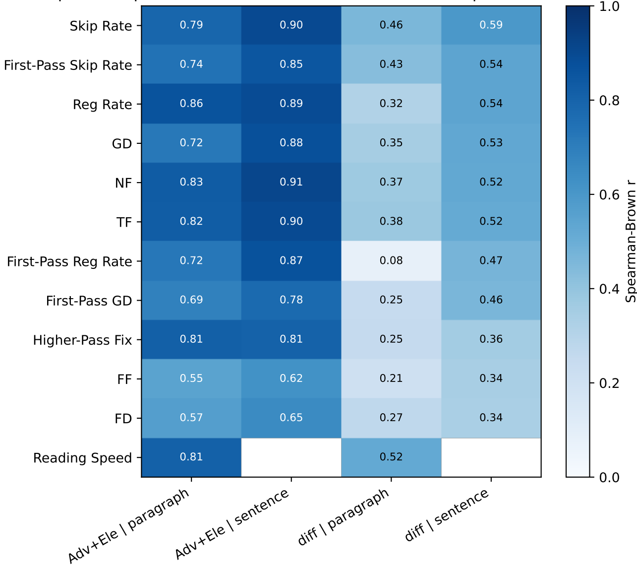
Split-half Spearman-Brown r — main+sm metrics — spearman — N=1000
