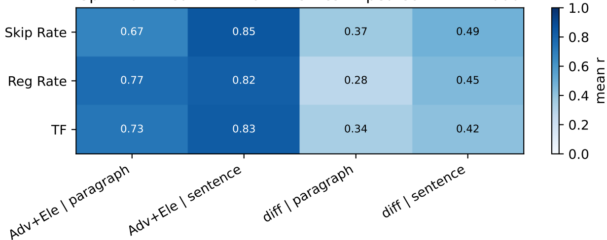
Split-half mean r — main metrics — pearson — N=1000
