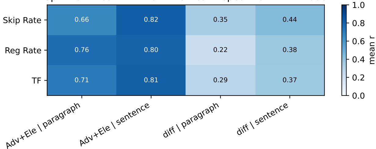
Split-half mean r — main metrics — spearman — N=1000
